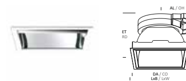
Wandfluter-Downlight, 4000 K, asymmetrisch / Wallwasher Downlight, 4000 K, asymmetrical
